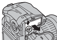
Akku-Schnappriegel
